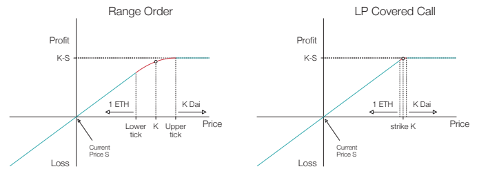
FIG. 1 Left: Deploying liquidity above the current spot price S (at origin) creates a range order which converts ETH to DAI as the price moves between the Lower and Upper ticks. The abscissa is the price of ETH vs Dai, the ordinate is the profit earned or the payoff curve, K is the price deployed to and serves as the strike price in the option-equivalent view. Right: Building on the left subplot, deploying liquidity to a narrow, single-tick range creates a “covered call-like” payoff where the ETH is sold immediately as the spot price crosses the strike K .
